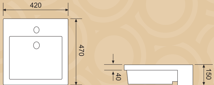
1 TH Square Style Recessed Basin
